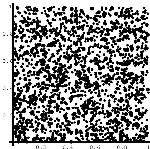
Graph I.1: Scatterplot of Two Independent Variables
