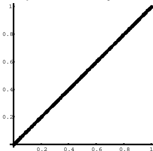
Graph I.2: Scatterplot of Two Perfectly Correlated Variables
